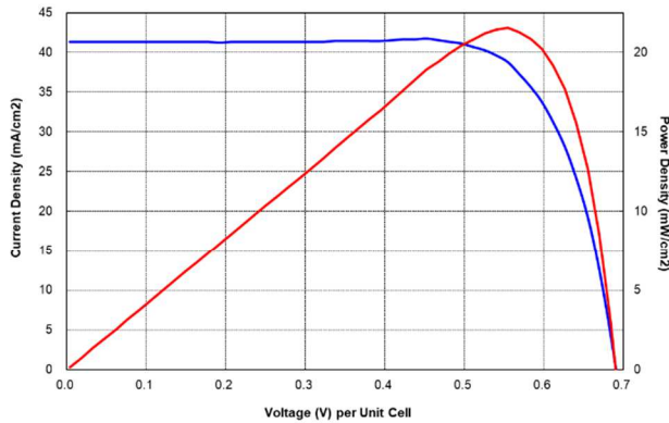
Current-Voltage Characteristics
