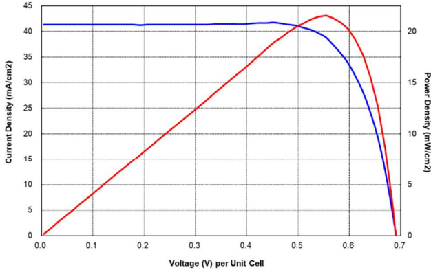
Current-Voltage Characteristics
