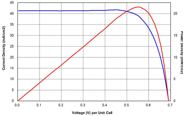
Current-Voltage Characteristics
