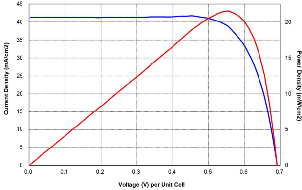
Current-Voltage Characteristics
