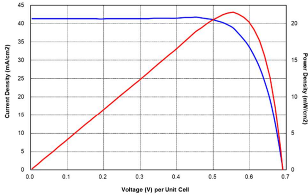
Current-Voltage Characteristics
