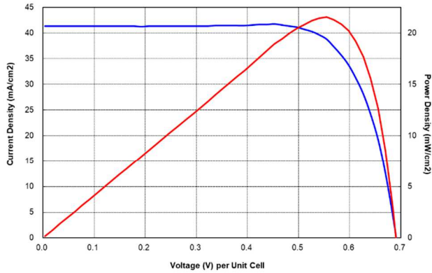
Current-Voltage Characteristics
